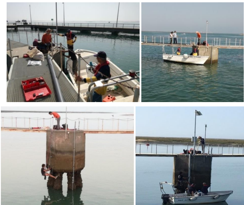
Figure 4.20. Installation of the online monitoring station: May 25 and 26, and June 23, 2017
