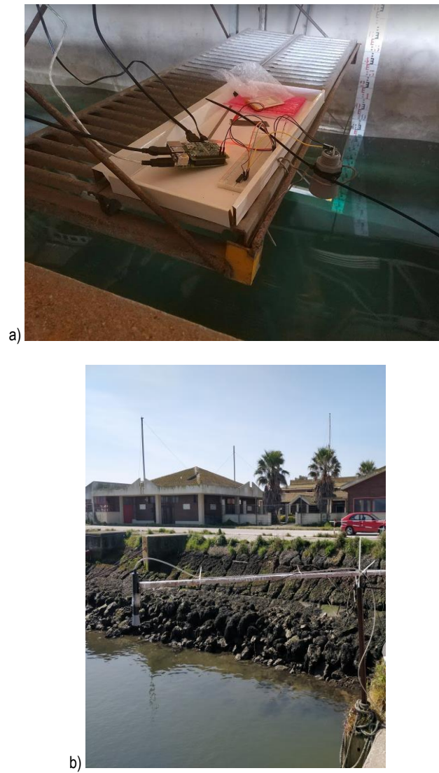
Figure 4.24 – Testing of the low-cost sensor for water levels: a) LNEC's wave flume; b) Mondego estuary site
