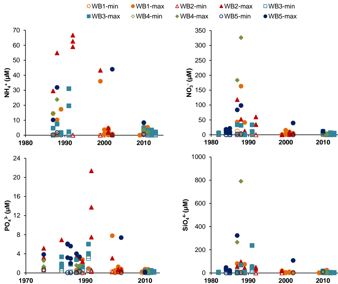
Figure 3.3 – Ammonium ( \text{NH}_4^+ ), nitrate ( \text{NO}_3^- ), phosphate ( \text{PO}_4^{3-} ) and silicate ( \text{SiO}_4^{4-} ) annual minimum and maximum concentrations between 1976 and 2013 (all data) in each water body of the Ria Formosa
